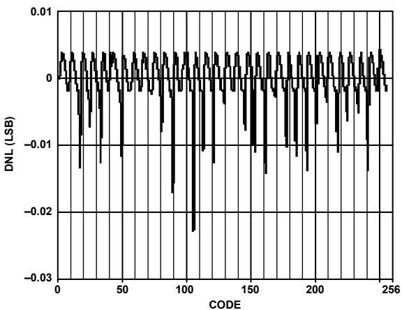
Figure 60. AD9704 Typical Uncalibrated DNL
