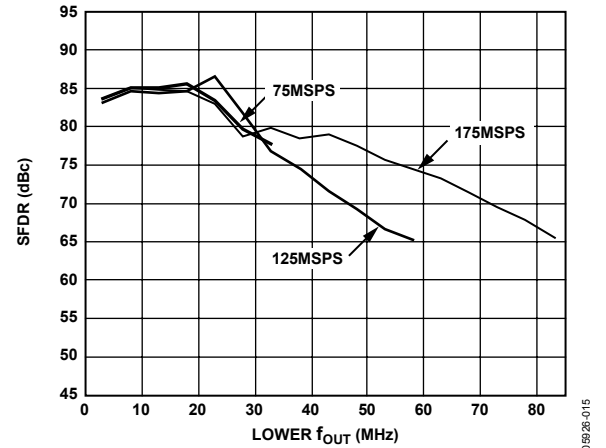
Figure 17. Dual-Tone IMD vs. f_{OUT} @ 0 dBFS
