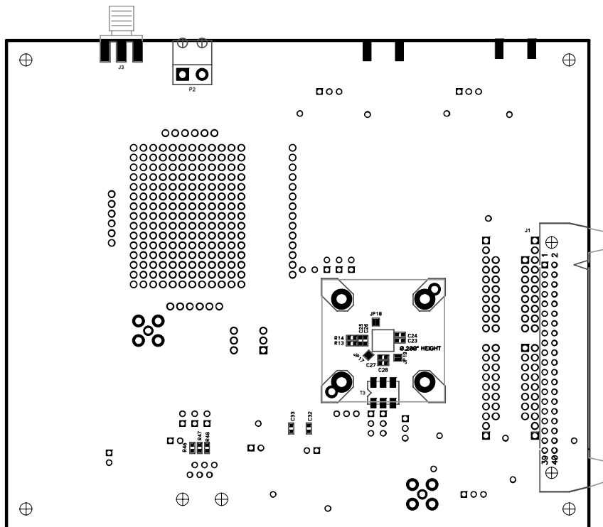
Figure 99. Assembly—Secondary Side
