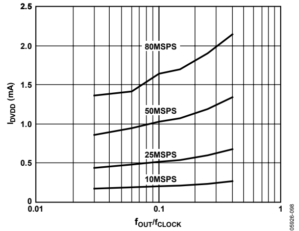
Figure 85. I_{DVDD} vs. f_{OUT}/f_{CLOCK} Ratio @ DVDD = 1.8\text{ V}
